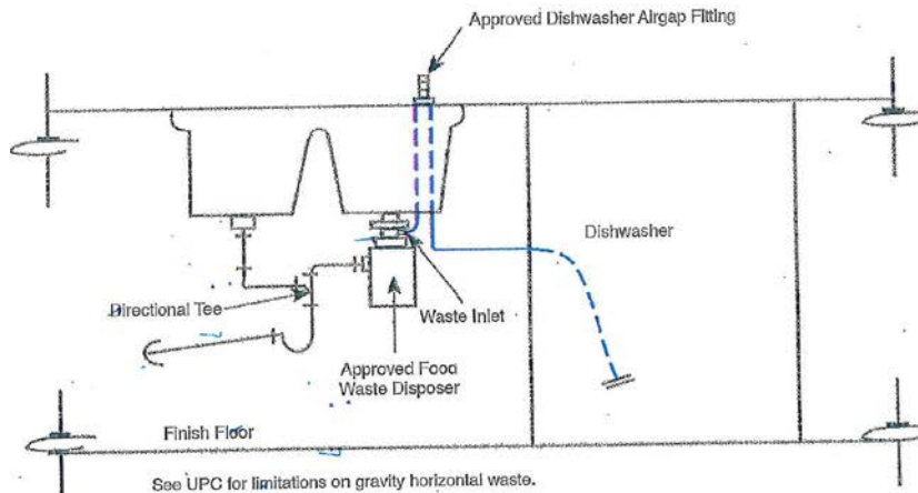
FIGURE 807.4A DISHWASHER AIRGAP CONNECTION THROUGH DISPOSAL
