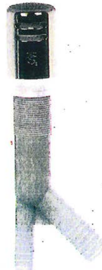
FIGURE 807.4B DISHWASHER AIRGAP CONNECTION THROUGH SINK TAILPIECE AND AIRGAP FITTING
