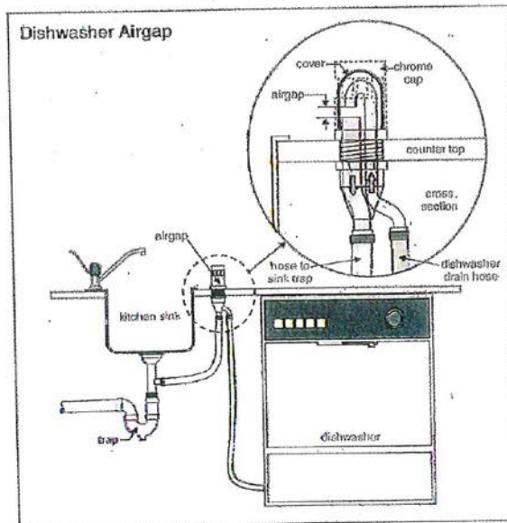
FIGURE 807.4B DISHWASHER AIRGAP CONNECTION THROUGH SINK TAILPIECE AND AIRGAP FITTING
