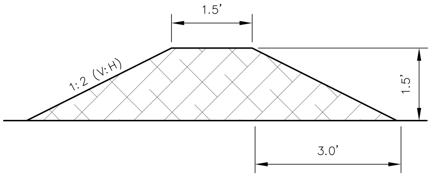
SECTION A-A BERM
