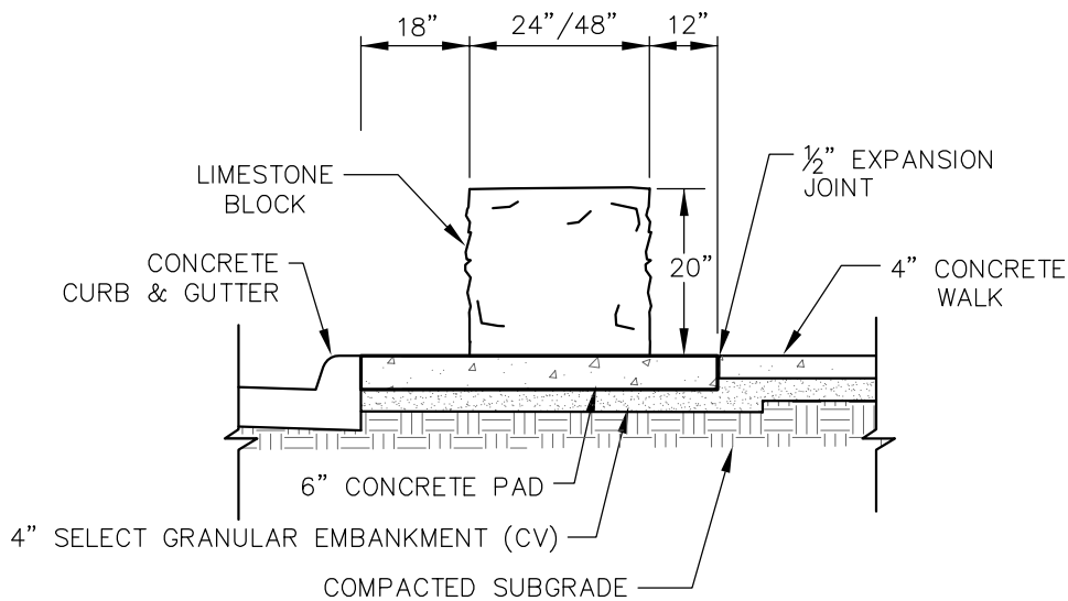
PROFILE VIEW
