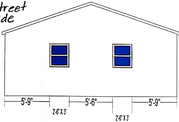
Gable Front View (2) - SINGLE HUNG (GOOD) 30X36
