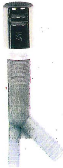
FIGURE 807.4B DISHWASHER AIRGAP CONNECTION THROUGH SINK TAILPIECE AND AIRGAP FITTING
