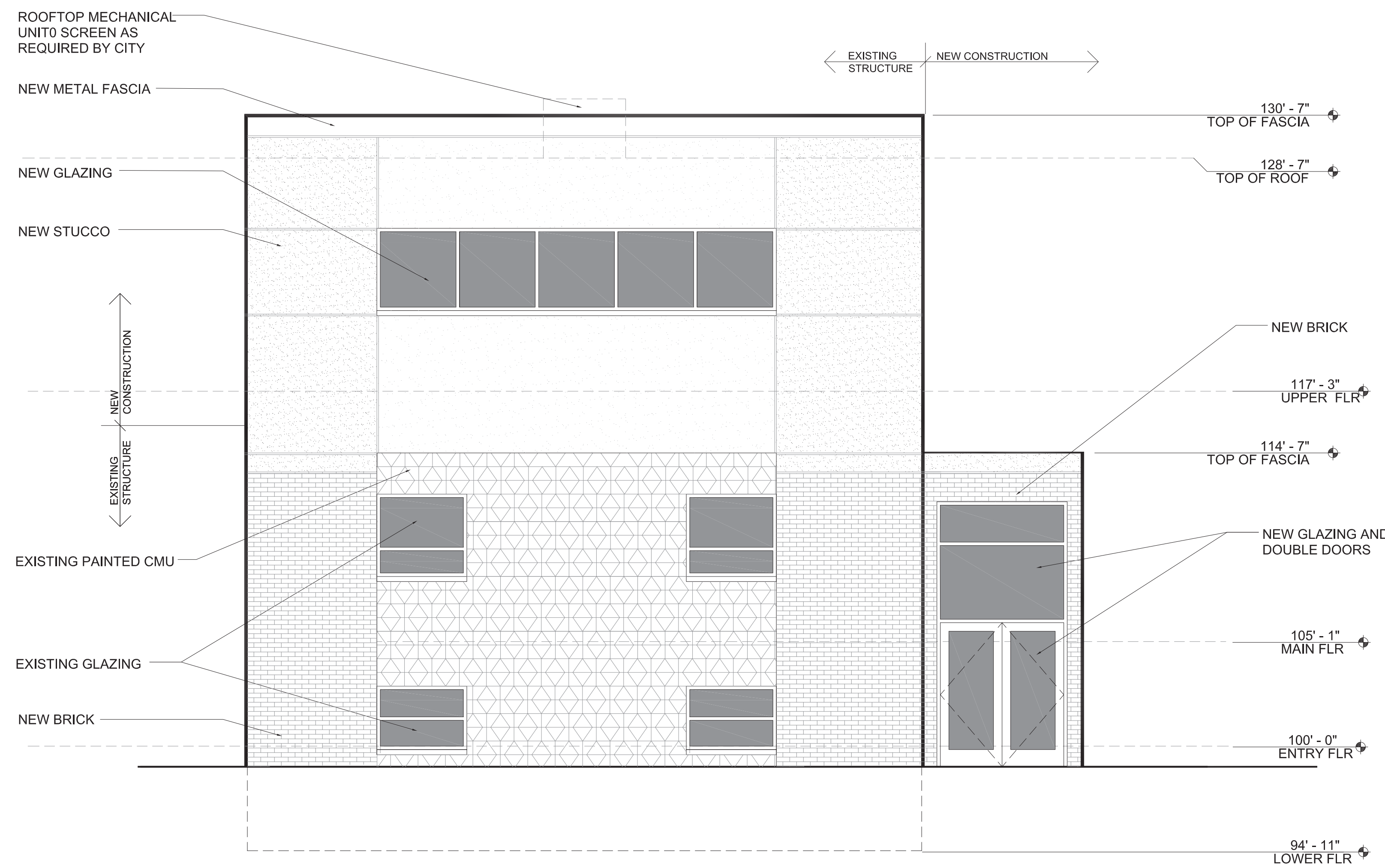
1 PROPOSED SOUTH ELEVATION A2.2 1/4" = 1'-0"
